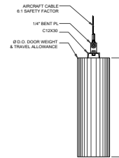
08 COUNTERWEIGHT TYP SCALE: 1-1/2" = 1'
