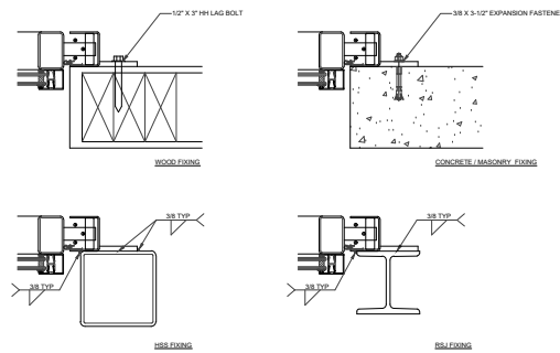
07 FIXING DETAILS TYP SCALE: 3" = 1'
