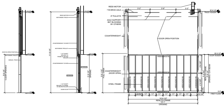
04 ELEVATION & SECTIONS MOTORIZED & NON SCALE: 1/4" = 1'
