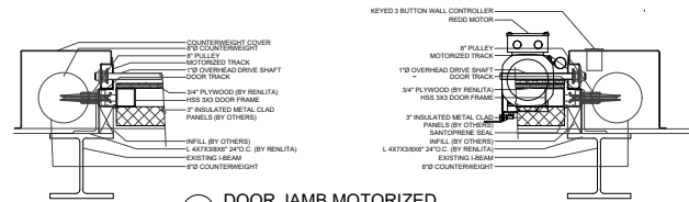
01 DOOR JAMB MOTORIZED SCALE: 1-1/2" = 1'
