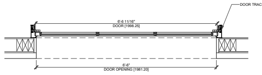
01 DOOR PLAN SCALE: 1" = 1'
