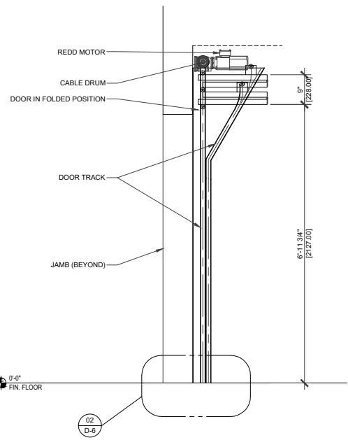
05 DOOR SECTION SCALE: 3/4" = 1'
