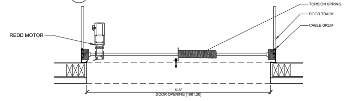
02 DOOR PLAN (ABOVE) SCALE: 1" = 1'
