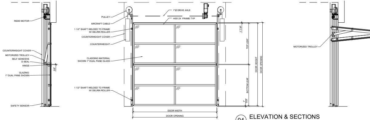
04 ELEVATION & SECTIONS SCALE: 1/2" = 1'
