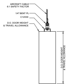
08 COUNTERWEIGHT TYP SCALE: 1-1/2" = 1'
